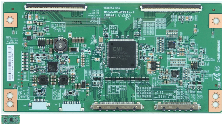
RCA LED55C55R120Q V546HK3-CS5 T-Con Control Board
