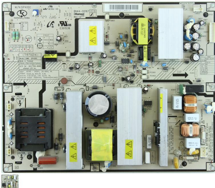
SAMSUNG LN-T4069F POWER SUPPLY UNIT BN44-00167C
