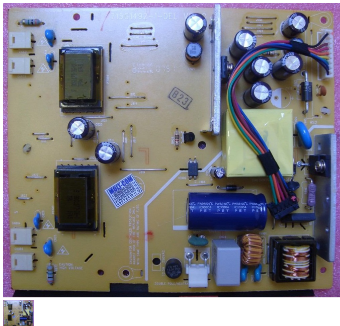
Dell E177FPC LCD Monitor Power board 715G1492-1-DEL
